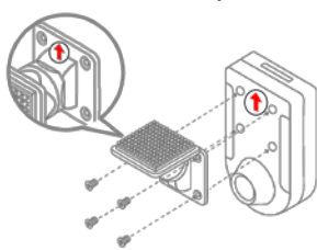
Use 4 screws provided to fix the 360° Mount to Recorder
